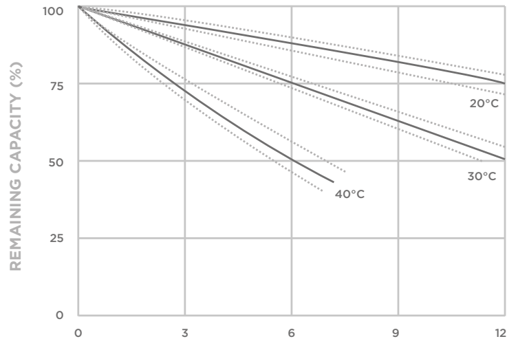
Figure 10 – Battery self discharge at varying temperatures
