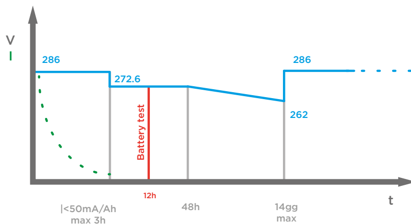
Figure 8 - Cyclic charging voltage plot
