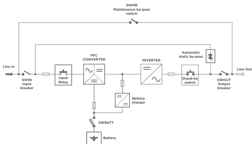
Figure 6 - Diagram of UPS with separate battery charger
