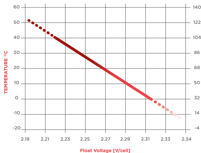
Figure 4 - Recommended cell charging voltage against temperature
