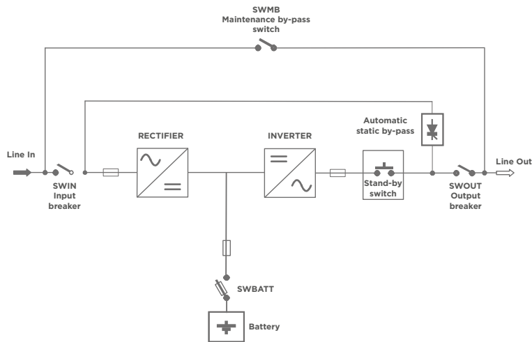
Figure 5 - Diagram of UPS with combined rectifier and battery charger
