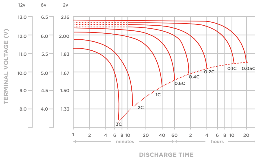
Figure 9 - Battery voltage discharge curve at varying discharge rates
